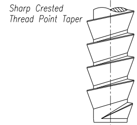
Sharp Crested Thread Point Taper Helical, Semi-Buttress 70°-10° Thread Profile
